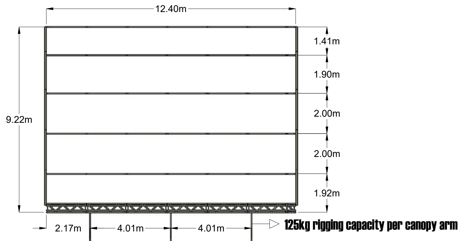
Rigging Structure - Top View
