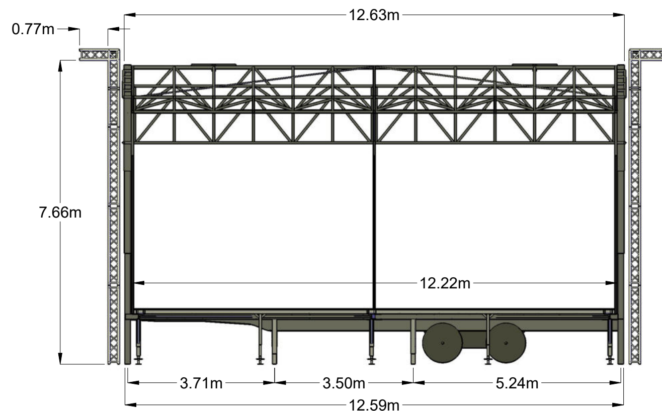
Front View
