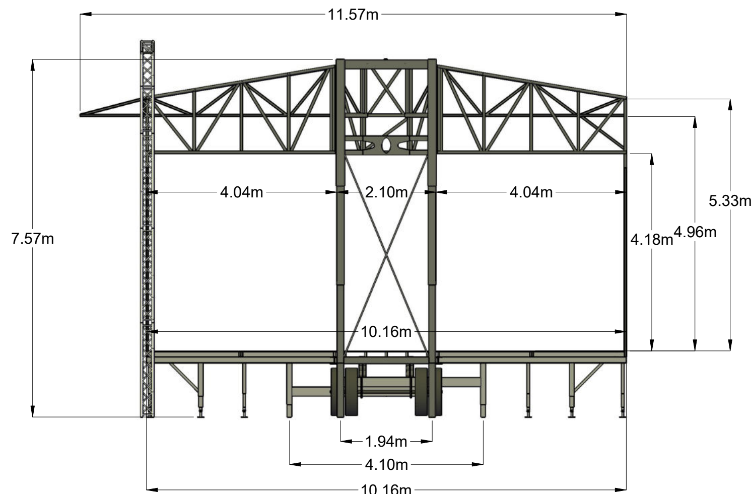
Side View
