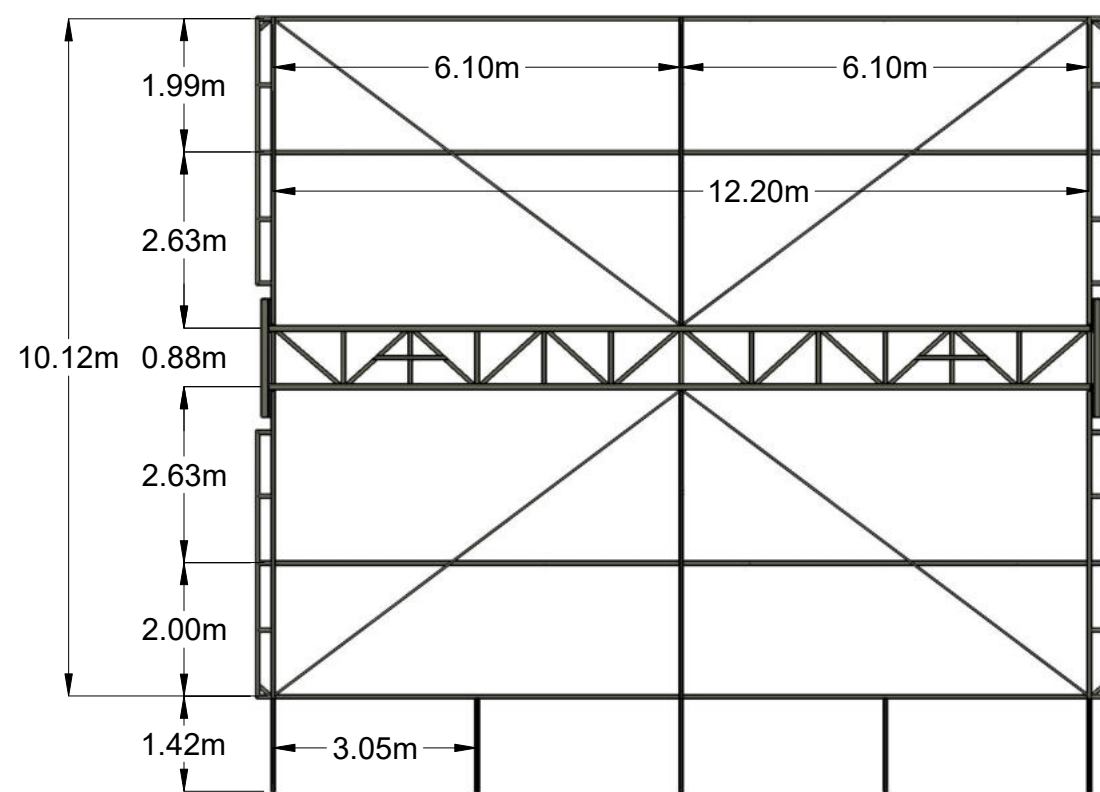
Rigging Structure
